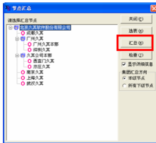
图6.1-4 节点汇总
